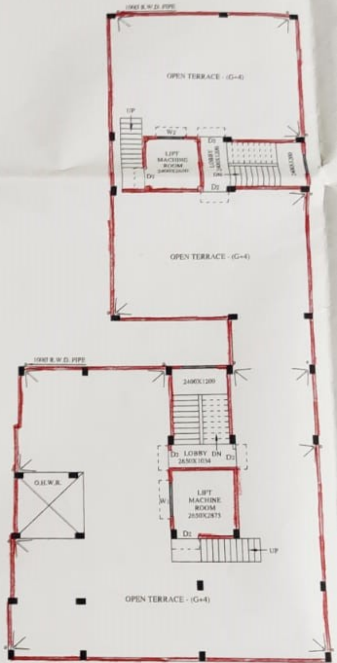
ROOF PLAN
